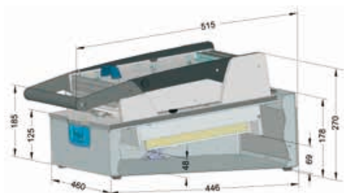
Detailed dimensional drawing of: MA 2112/D/H/S-7 with ATS 2112/S-7
